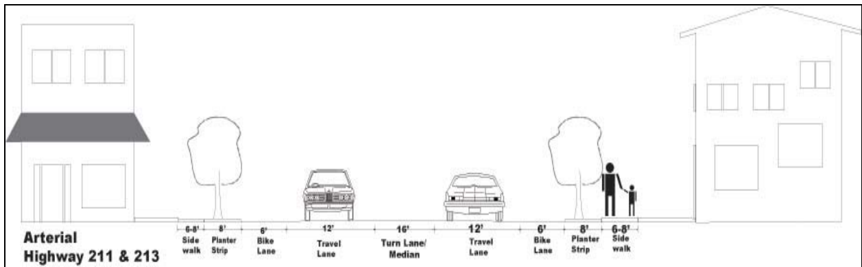
Figure 18.4.100(F.9) Arterial (Highway 211 & 213) Street Section
