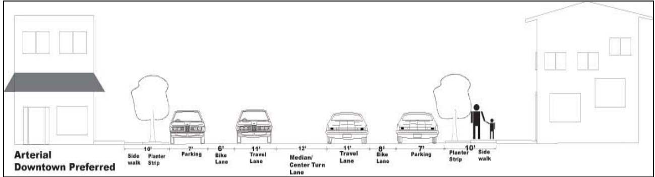
Figure 18.4.100(F.7) Arterial (Downtown Preferred) Street Section
