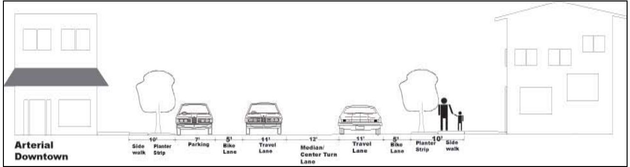
Figure 18.4.100(F.9) Arterial (Highway 211 & 213) Street Section
